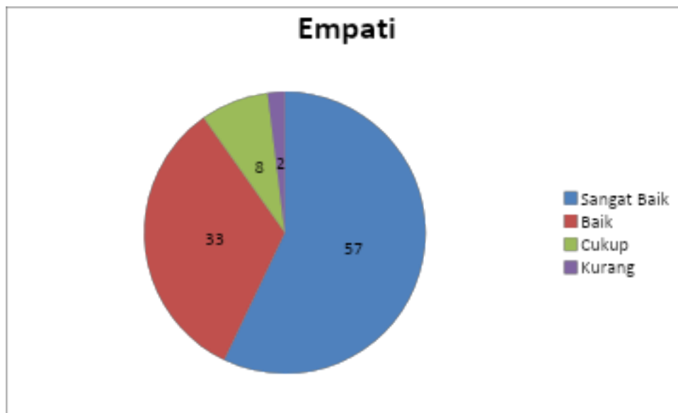
Gambar 4: Emphaty
